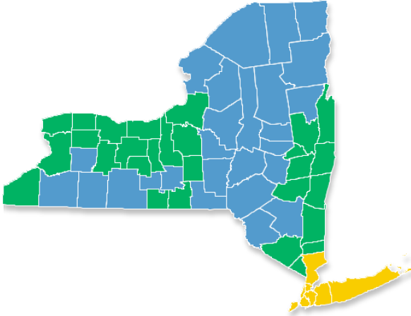
Figure 1. New York State Climate Zone
